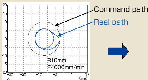
Radius shrinkage 4mm
