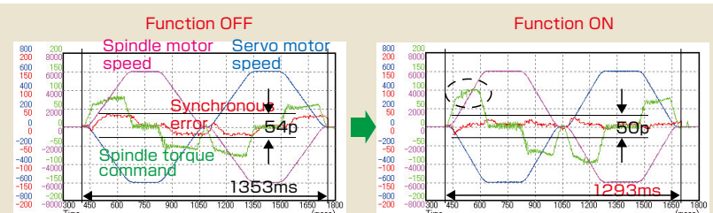
FSSB High-speed rigid tapping (Example)
