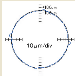
Protrusion 6μm
